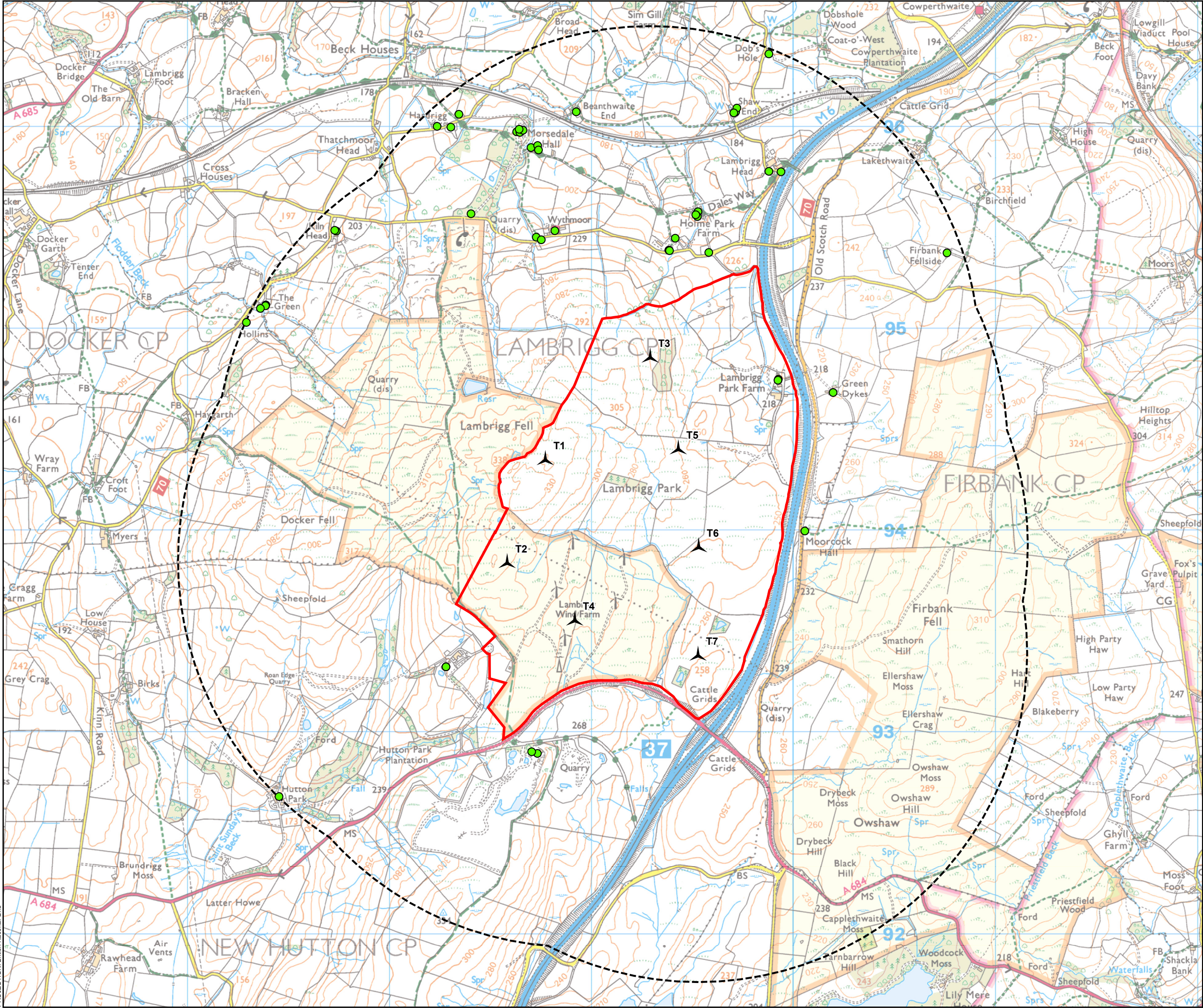
Figure 15.1 Shadow Flicker Study Area
