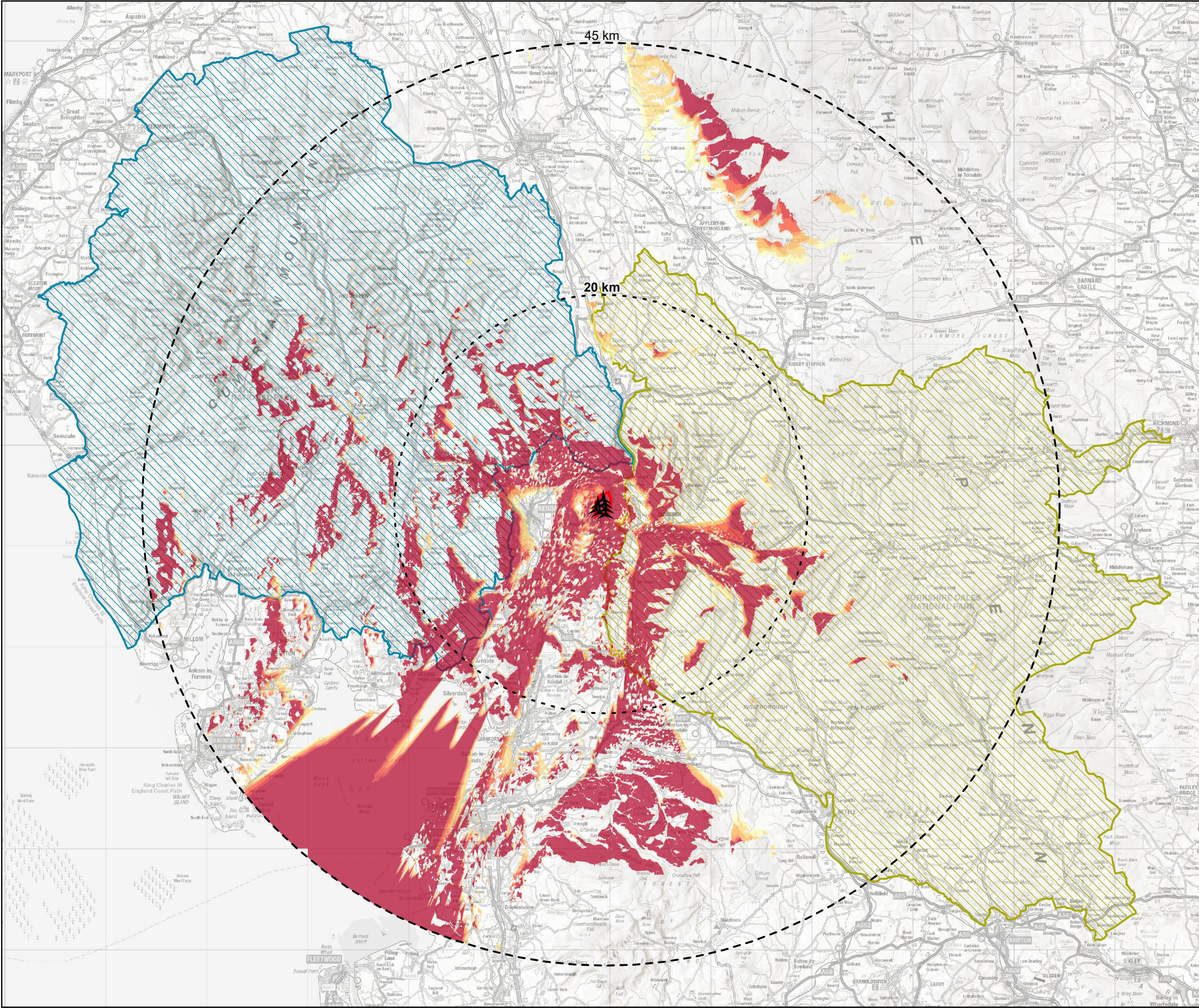
Figure 5.5 Turbine Blade Tip Height Zone of Theoretical Visibility to 45 km
