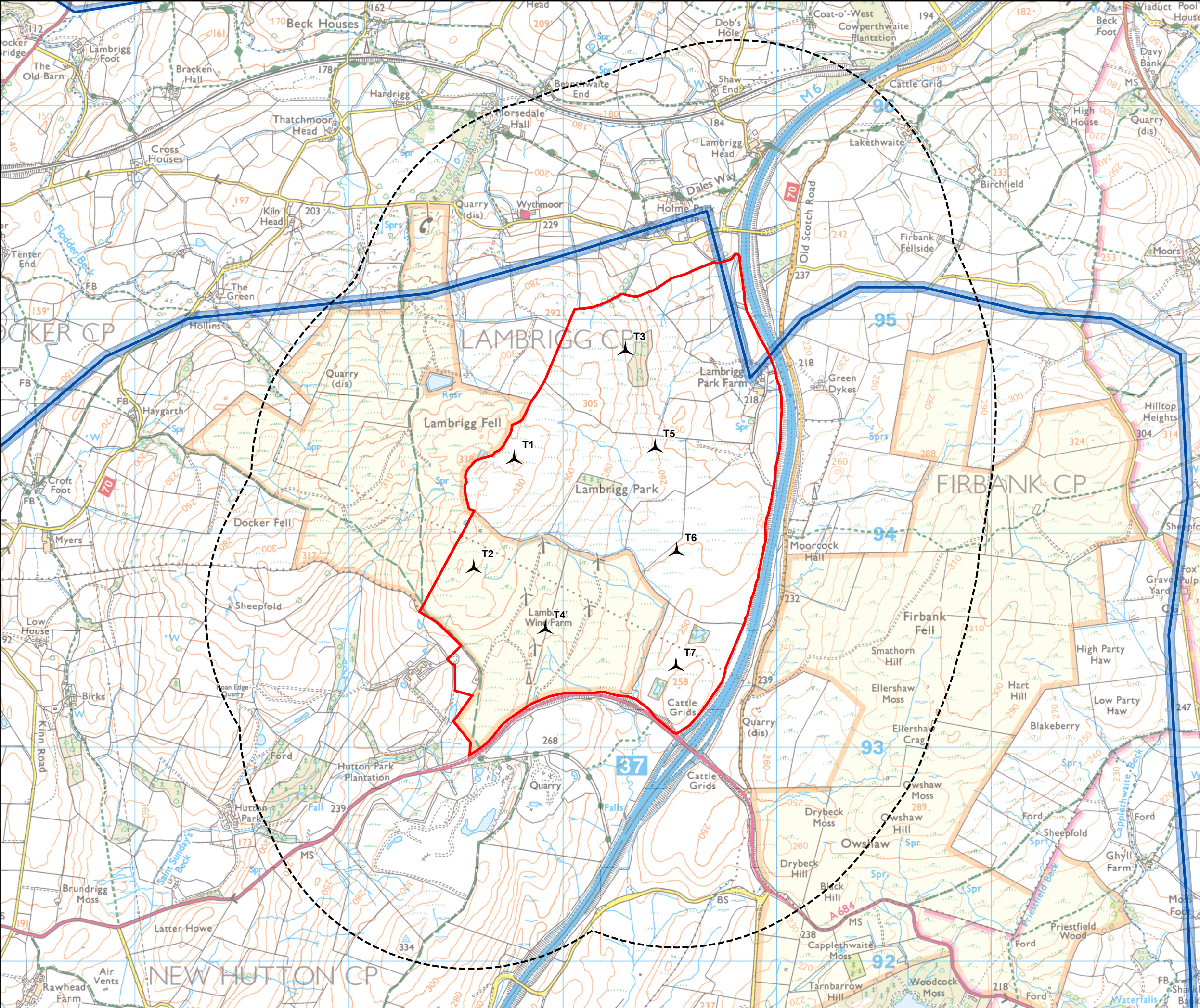
Figure 9.3 Hydrogeology
